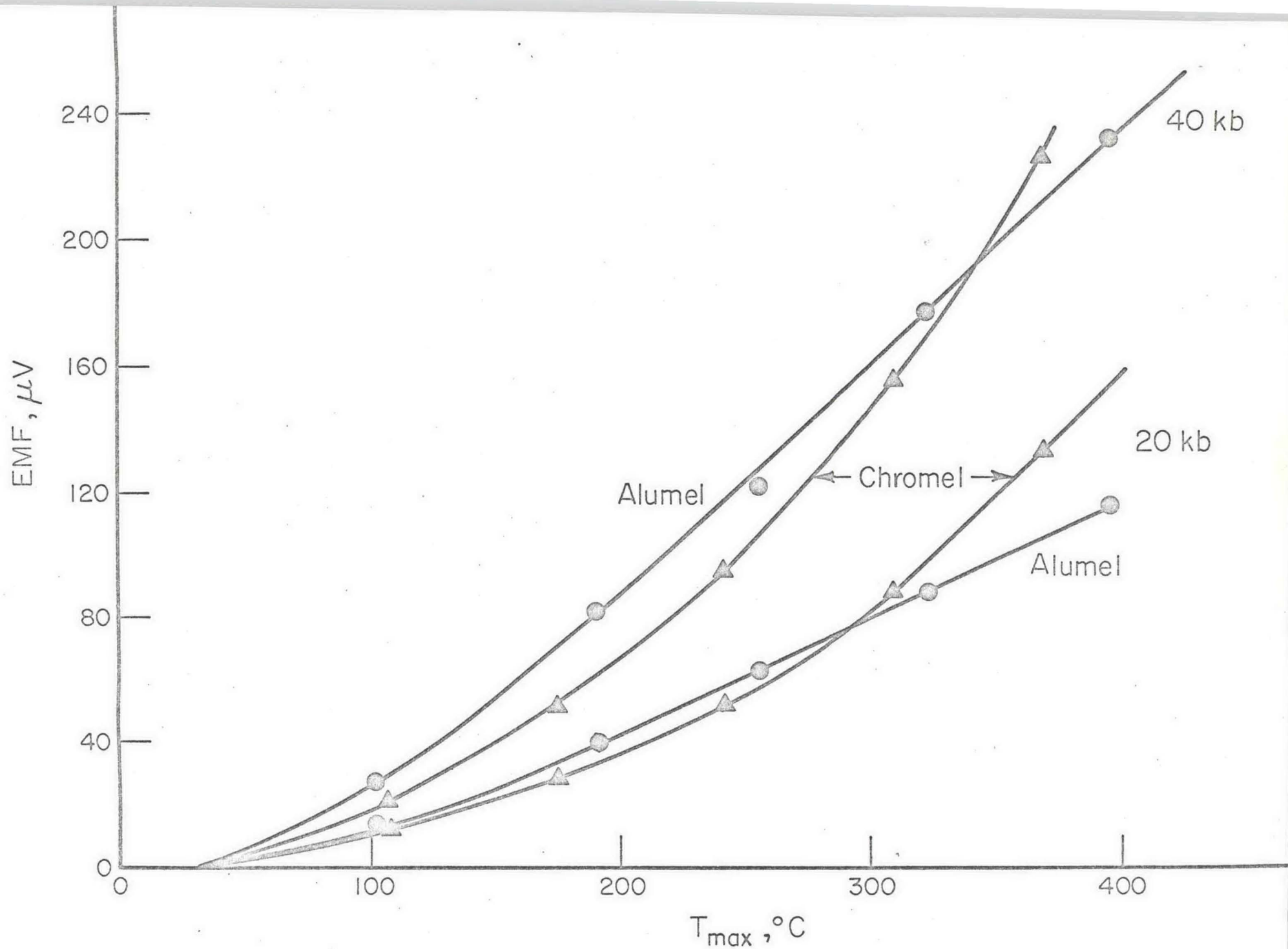
PRESSURE EMF VERSUS TEMPERATURE CHROMEL-ALUMEL Cold + ; hot -
